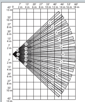
5800PIR-COM Top View
